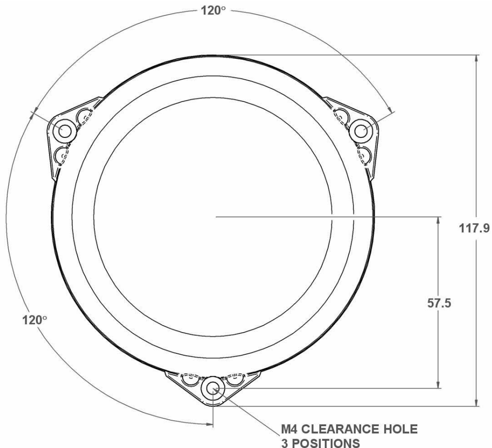
Figure 2 - SAT-201 M4 Drilling Diagram (not to scale)
